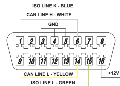
CONNECTOR FRONT VIEW
